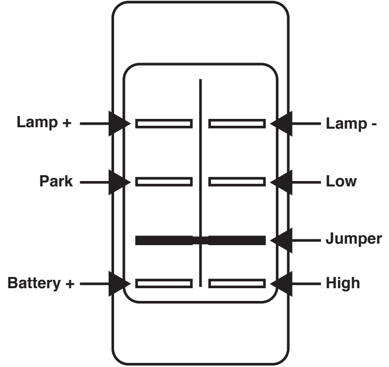
Dynamic Park Wiring
