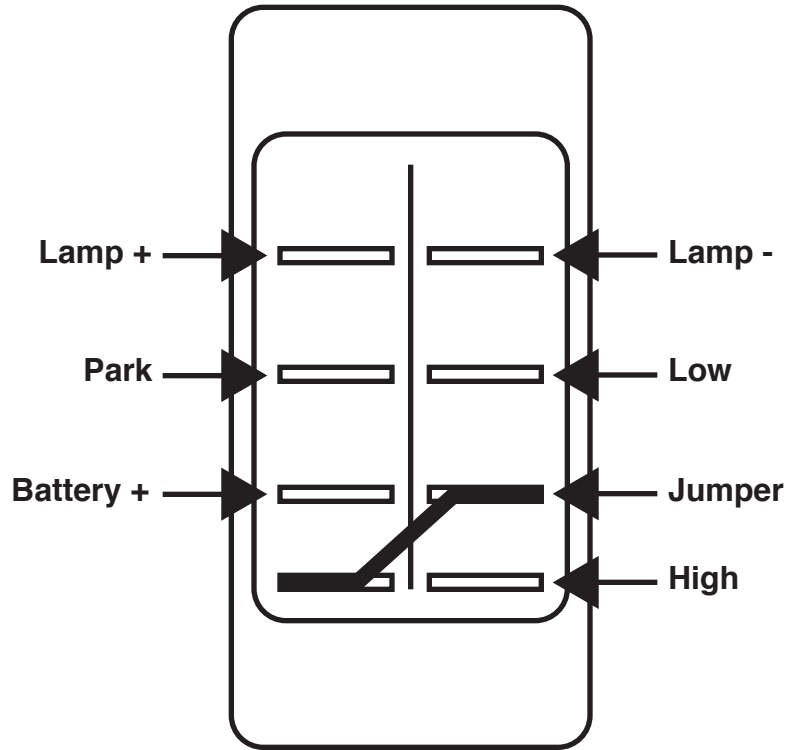
Coast to Park Wiring
